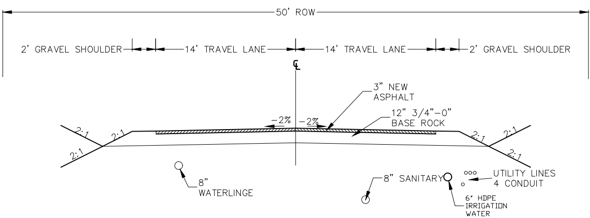
TYPICAL SECTION 4-4 NTS
