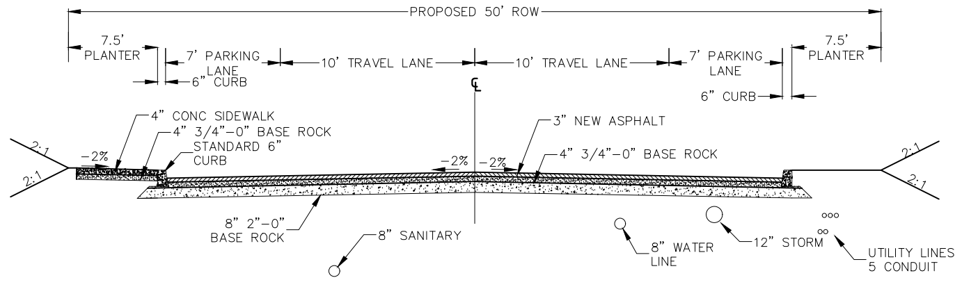
TYPICAL SECTION 6-6 NTS
