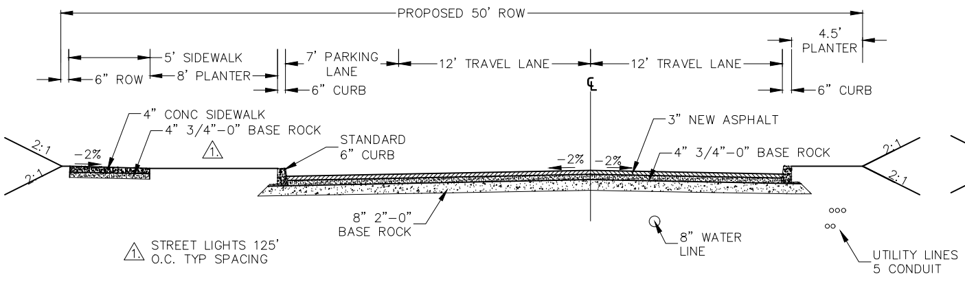
TYPICAL SECTION 7-7 NTS
