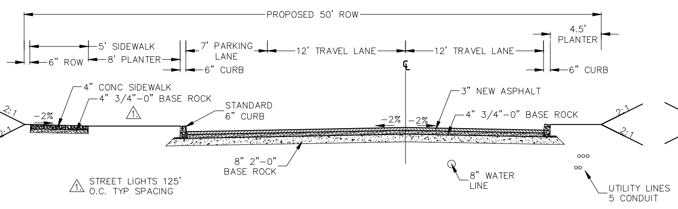
TYPICAL SECTION 7-7
