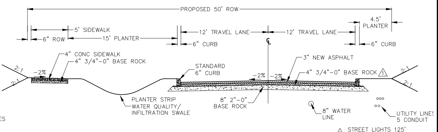
TYPICAL SECTION 8-8
