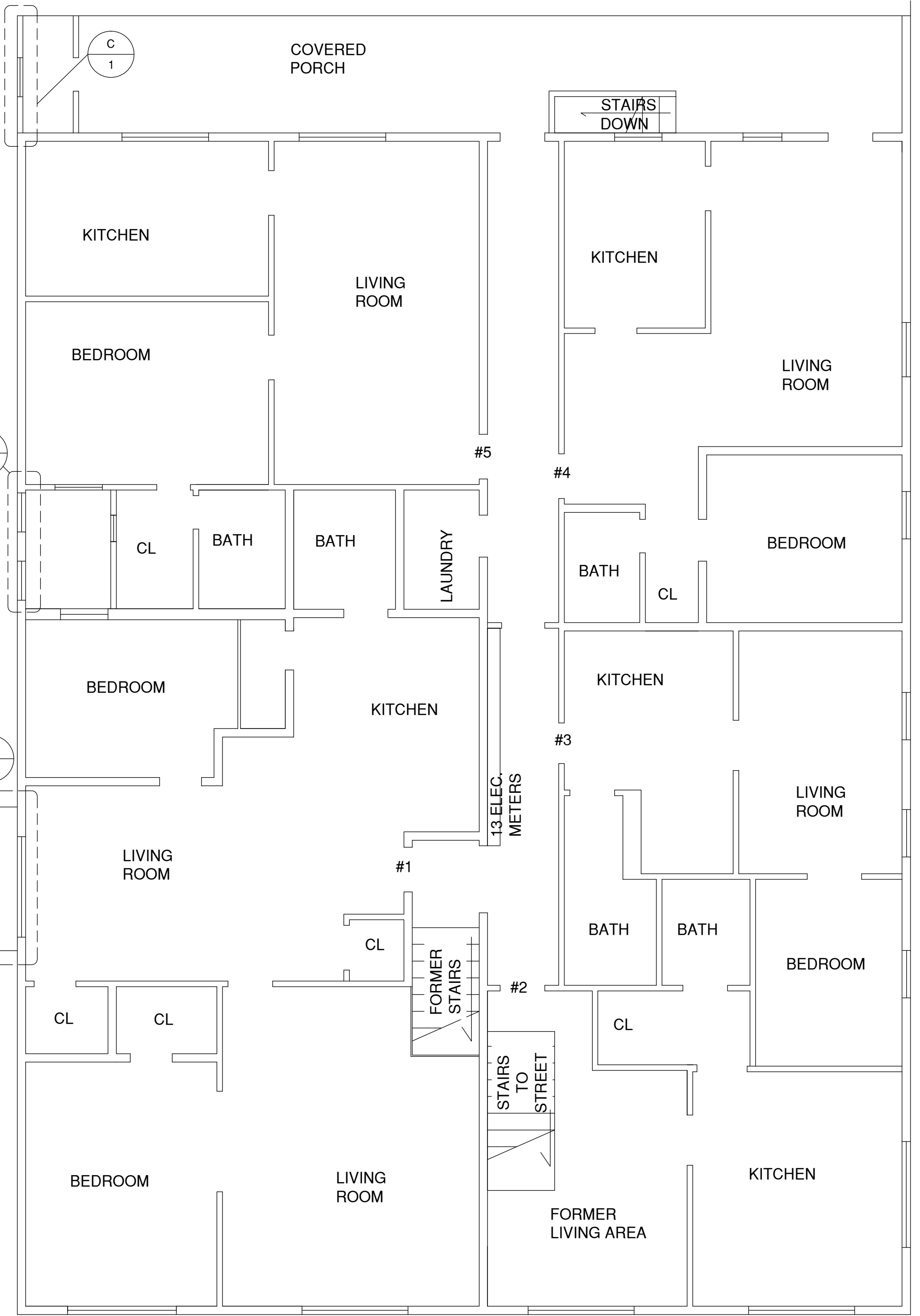
FLOOR PLAN Approximate Scale: 3/32":1'-0"
