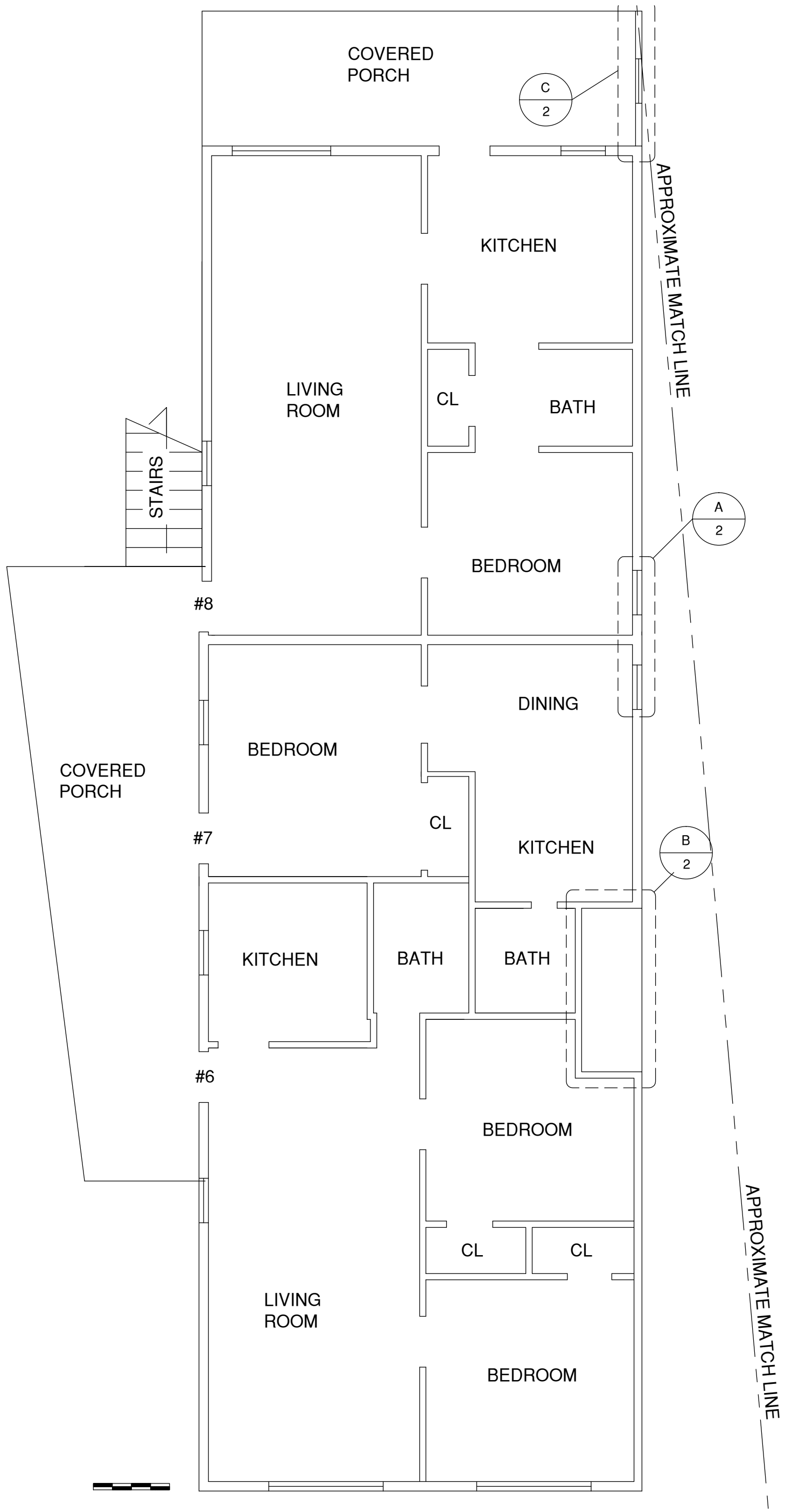
FLOOR PLAN Approximate Scale: 3/32":1'-0"
